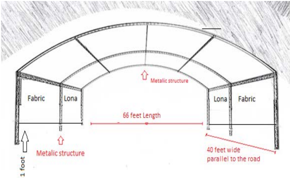
Figure 2. Design and size. Lateral fabric must be be one (1) foot up above floor level.
